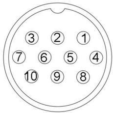
Socket viewed from solder side
