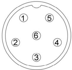
Socket viewed from solder side
